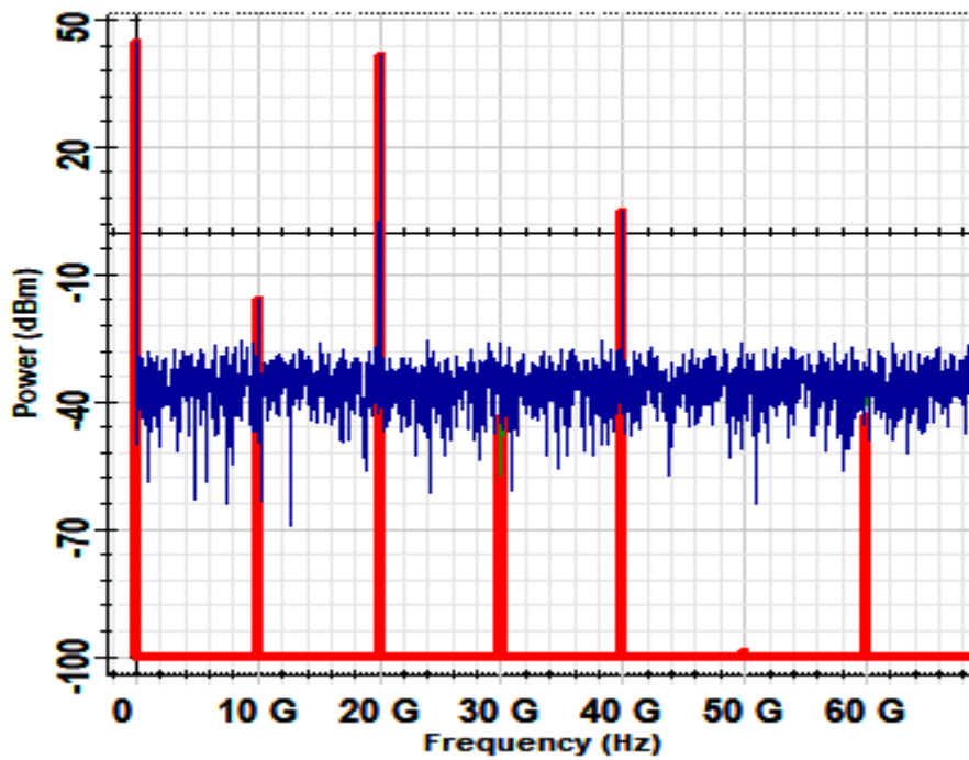
Signal plus noise RF spectrum
