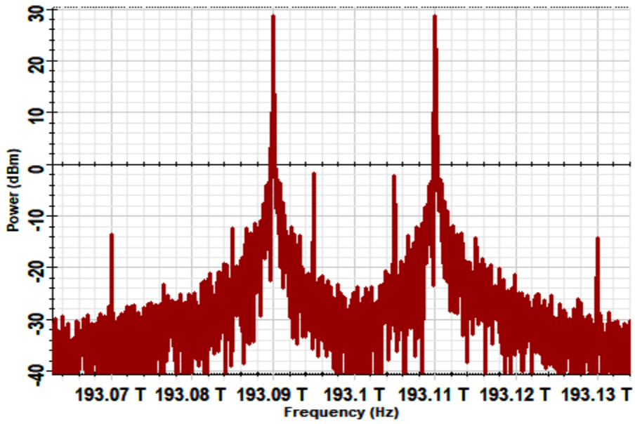
Optical spectrum to be beaten by photodiode
