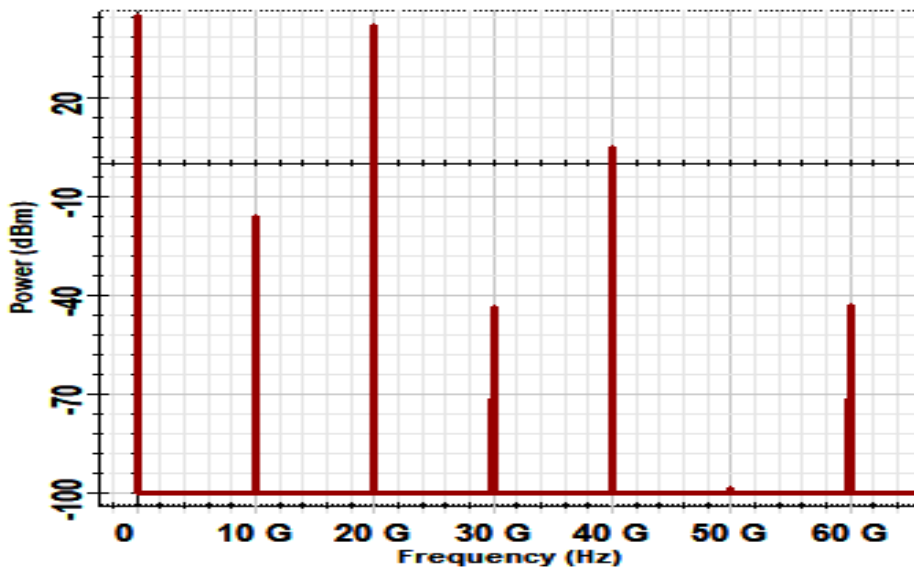
Signal only RF spectrum
